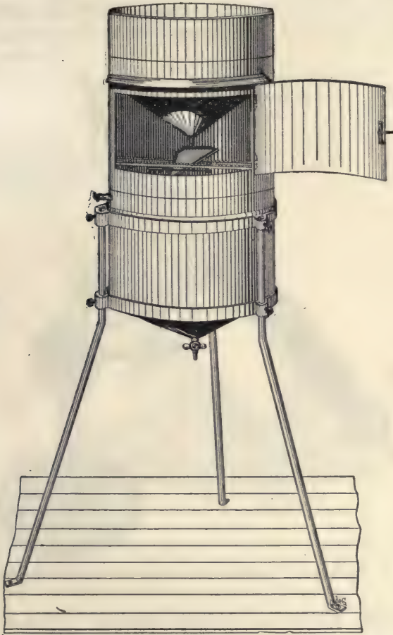
FIGURE 17. Tipping-bucket Rain-gauge.
